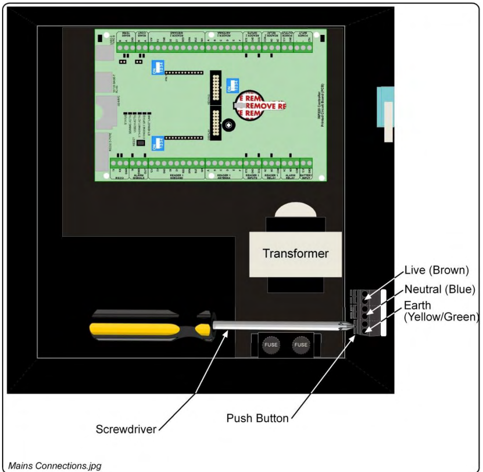
Figure 14: Mains Connections
