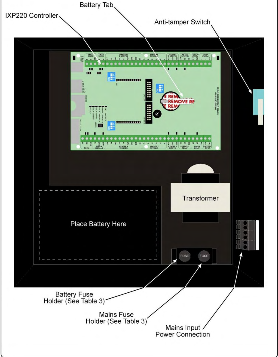
Figure 5: Power Supply Combo Layout
