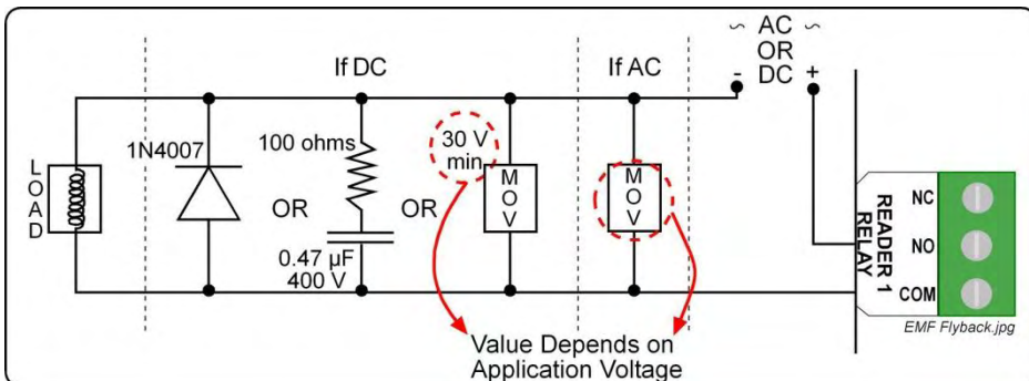
Figure 2: EMF Flyback
