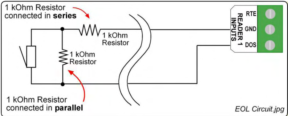
Figure 1: End of Line (EOL) Sensing Circuit
